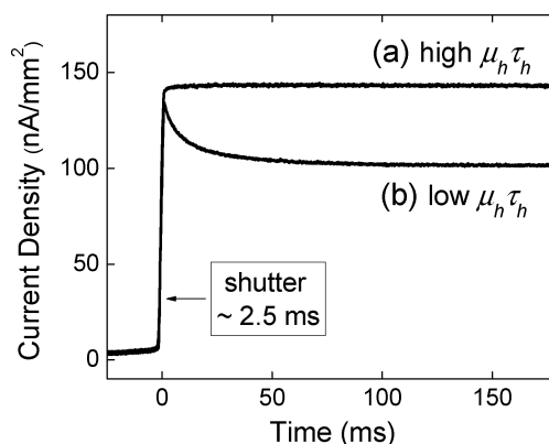
Fig. 1. X-ray photocurrent temporal response from planar, 2 mm thick CdZnTe detectors at 300 V bias: (a) high \mu_h\tau_h material, (b) low \mu_h\tau_h material.
