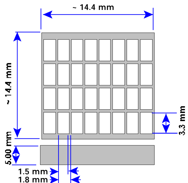
Figure 1. Pixel configuration and typical dimensions of the individual CZT crystals.
