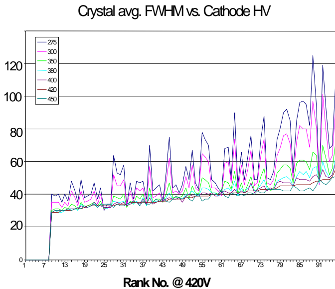
Figure 3. Energy resolution of individual crystal as a function of the applied voltage on the cathode. Ranking of crystals has been obtained at 420 V and maintained for all the other curves, Vertical axis in FWHM of energy resolution x 10. At 420 V the average of ALL crystals is below 6%
