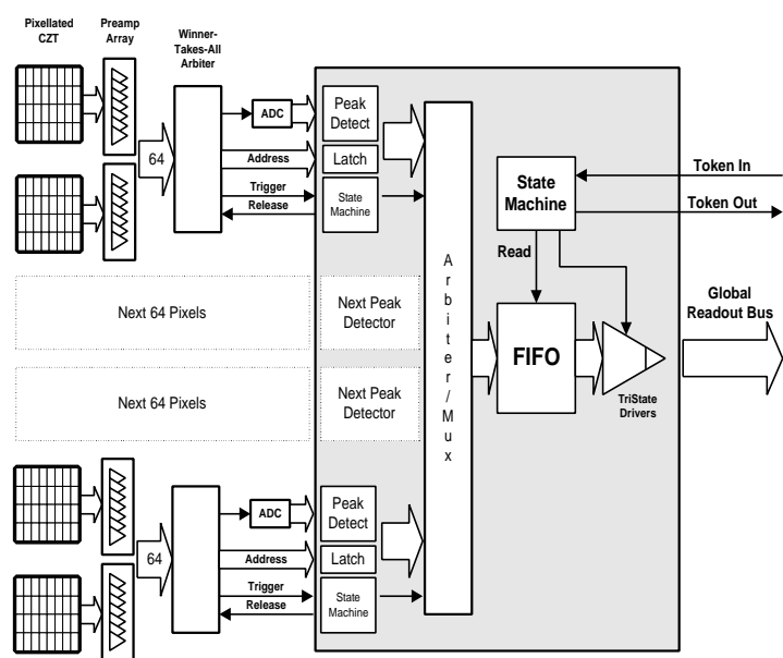
Figure 2. Basic functions and data flow/data reduction in the Solstice camera. With the current architecture and dead time characteristics, several millions counts per second can be achieved with the detector without any loss in performance.
