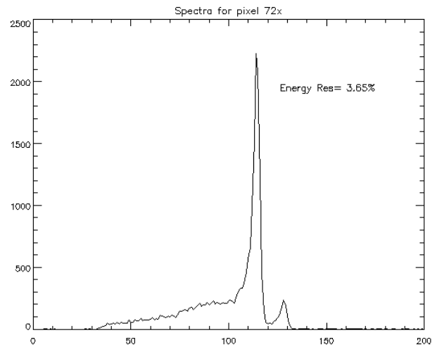
Figure 4. Energy spectrum for pixel 72x measured at 3.65% FWHM for 57 Co
